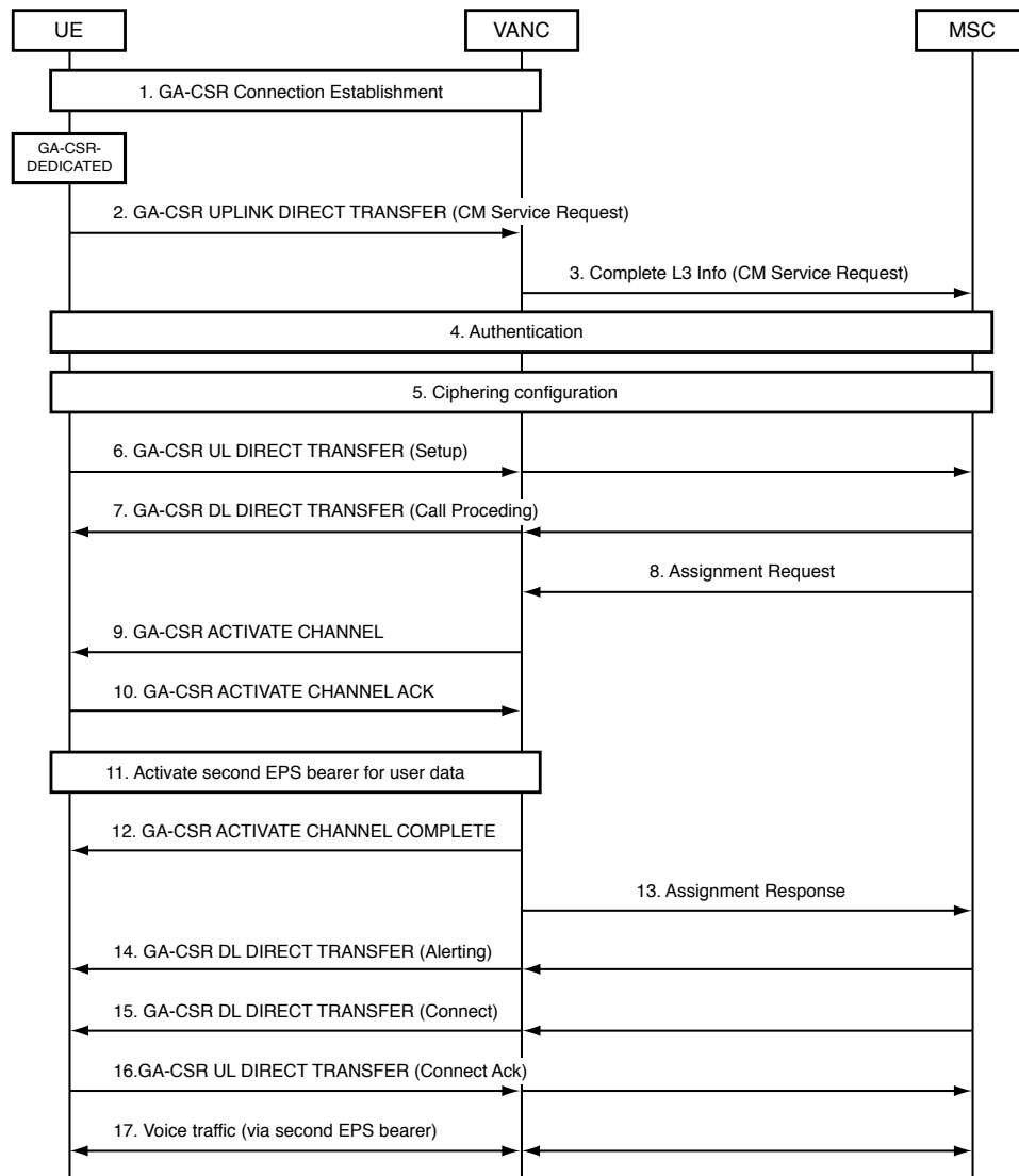
Figure 2.2: Call flow for a mobile originated voice call (VoLGA stage 2 specification, Figure 9.8-1)
