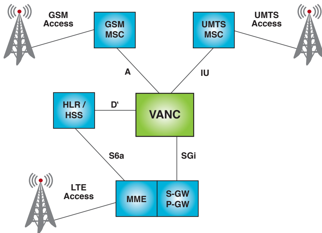
Figure 2.1: Basic VoLGA network setup
