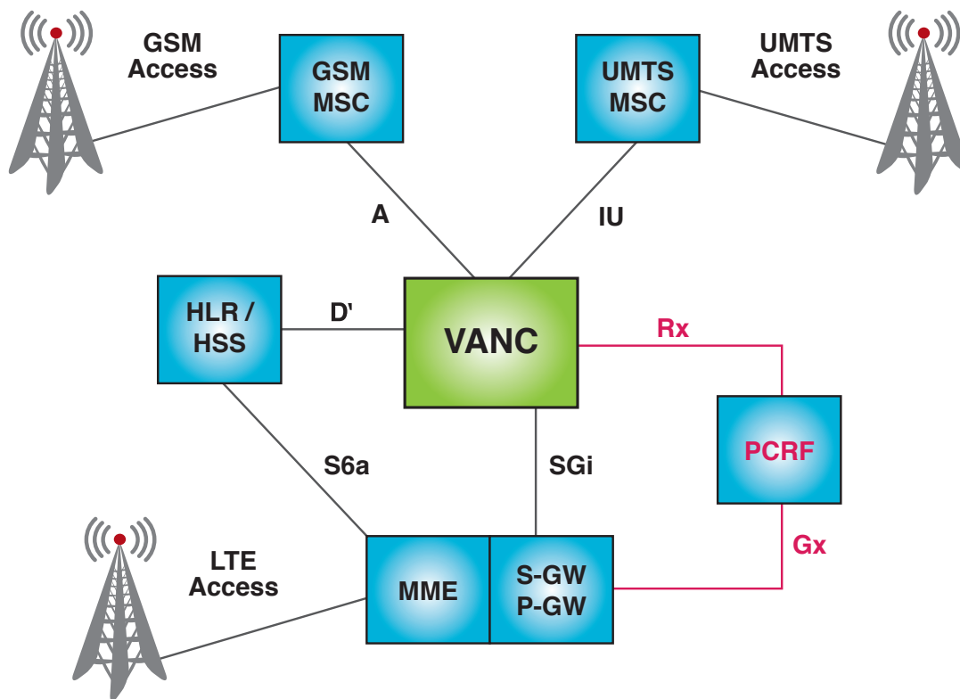
Figure 2.4: Ensuring Quality of Service for the Voice Call with the PCRF
